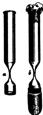
Fig. 80.—Preparation of collodion sacs: a , Test-tube constricted and cut; b , sac attached to the tube.
